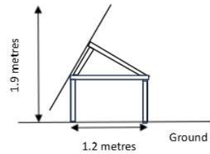
Figure 3 East/Side Elevation
